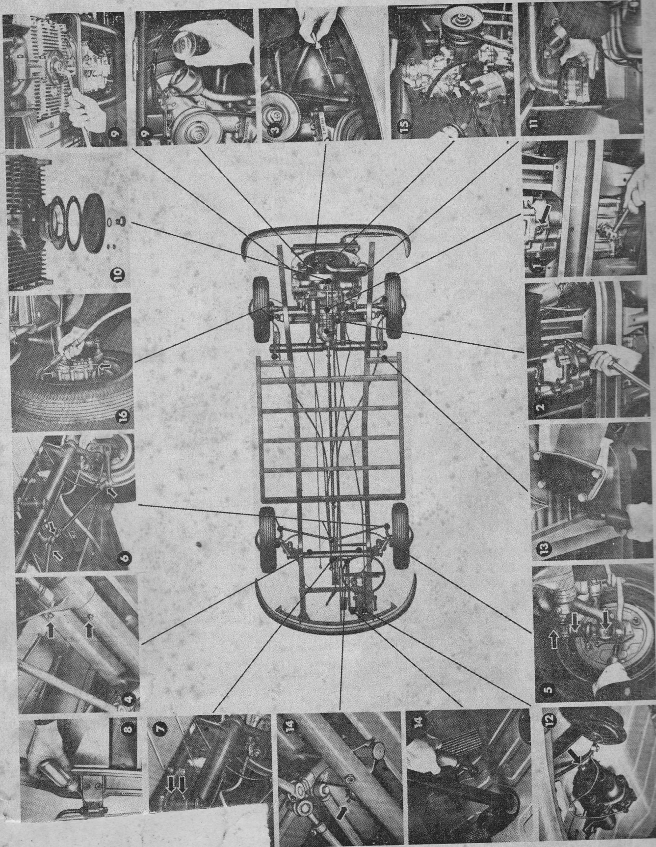
Lubrication points for the Transporter.
